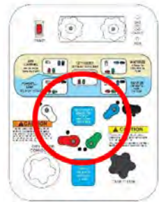
Fig 3: Set 3 valves to 45°
